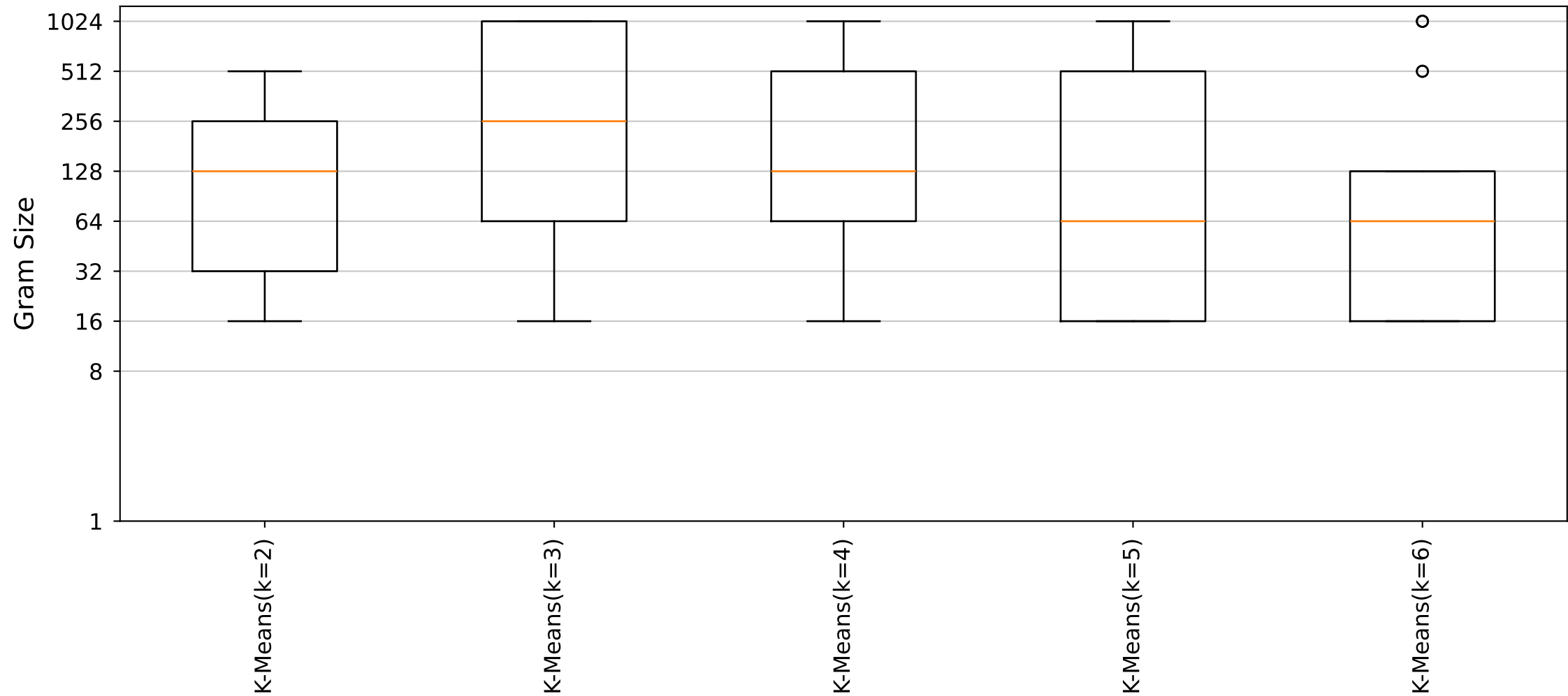
YARA Rules Gram Size Distribution (Cluster28_Size6 dataset)
